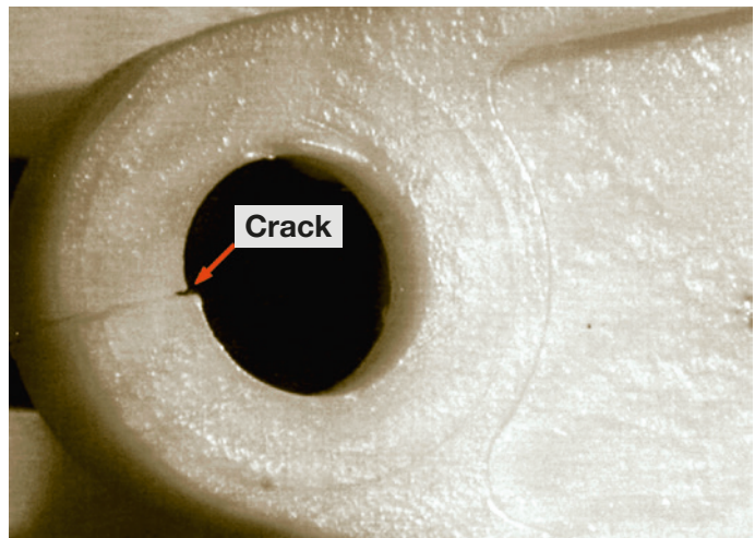
Figure 4, POM clamp ( M = 18 , AL). Through the gate area (left eye), a crack develops in the weld line, and the molded part surface shows a very cold impression of the mold surface (see also → weld line and → orange skin).
