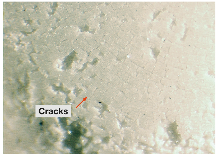
Figure 7, PA/PTFE sheet (M = 1 : 1) with samples and microcracks after media exposure and a weathering dose of 15,000 MJ/m 2 in a Xenon tester 1200 CPS. The insular microcrack formation was also benefiting from an increased molded part stress in the surface due to shrinkage stresses and a too-rapid cooling in injection molding.
