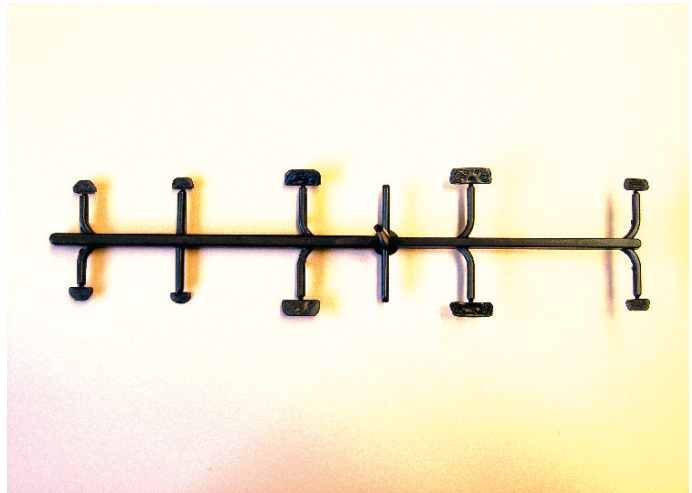
Figure 3, PA/PTFE runner ( M = 1 : 1 ) with 10 mold cavities and symmetry balance through polishing. The molded part quality improves in all 10 cavities through balancing the gates in the runner. For this, the gates were partially polished to varying degrees because different flow path lengths are present between the direct gate and the mold cavities. The goal was an equally fast filling of the mold cavities.
