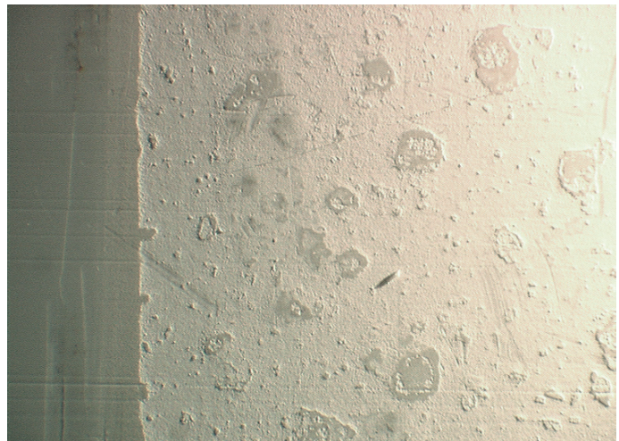
Figure 8, PVC-U window profile (M = 31, AL) with weathered surface after 8000 MJ/m 2 in a Xenon tester beta LM. The original surface can still be detected on the left side of the figure (see also Fig. 9).
