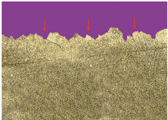
Figure 12, PP lounge seat (M = 100, AL) with UV stabilization. A rough PP surface developed after four years of outdoor weathering in Würzburg, Germany. Thus the dirt deposits cannot be removed with the cleaning products that were recommended by the manufacturer, and the rough PP surface retained a gray appearance.
